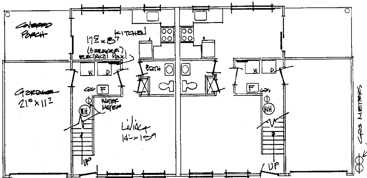
FIRST FLOOR
