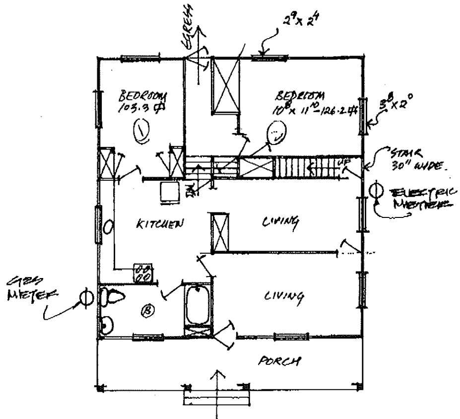
122 NORTH COLLEGE FIRST FLOOR PLAN INSPECTED - 9/07/93
