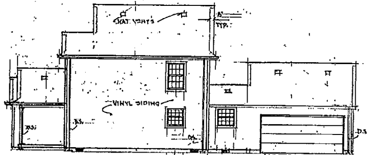
RIGHT (EAST) ELEV. 1/8" = 1'-0"
