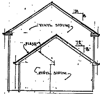
REAR (NORTH) ELEV. 1/8" = 1'-0"
