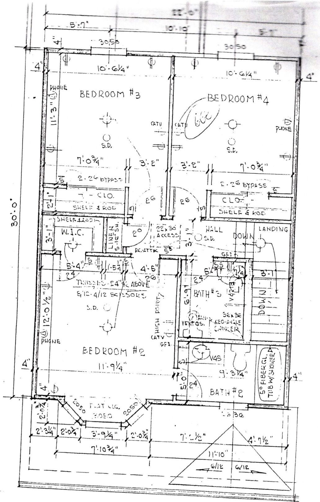
2 ND FLOOR PLAN 1/4" = 1'-0" 672 SQ. FT.
